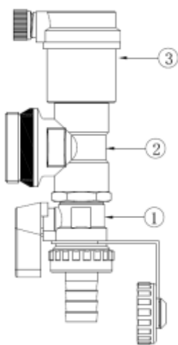
①-Drain valve
