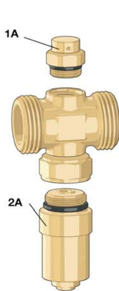
Antifreeze valve
