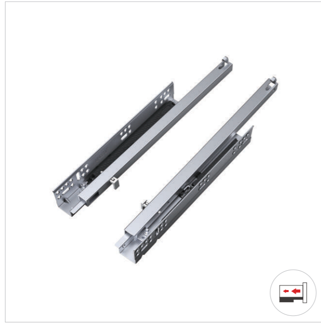
名称 半拉出二节(阻尼)隐藏轨 调整钉插销款 Name (SOFT CLOSING) SINGLE EXTENSION UNDERMOUNTED SLIDE WITH ADJUSTABLE PIN
