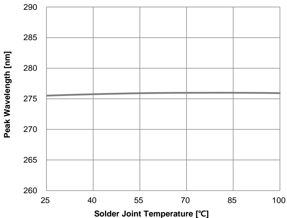
Fig 6. Solder Joint Temperature vs. Peak Wavelength, I_F=30\text{mA}
