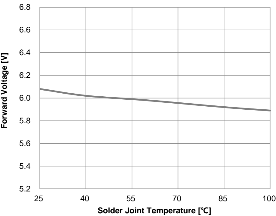
Fig 7. Solder Joint Temperature vs. Forward Voltage, I_F=30\text{mA}
