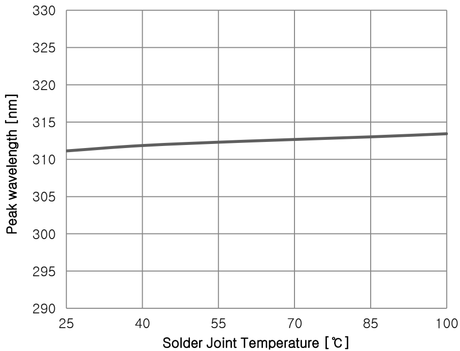
Fig 6. Surface Temperature vs. Peak Wavelength, I_F=20mA
