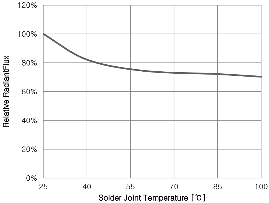
Fig 5. Surface Temperature vs. Relative Radiant Flux, I_F=20mA
