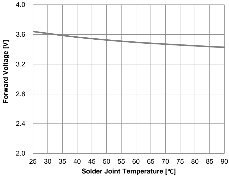
Fig 7. Solder Joint Temperature vs. Forward Voltage, I_F=250\text{mA}
