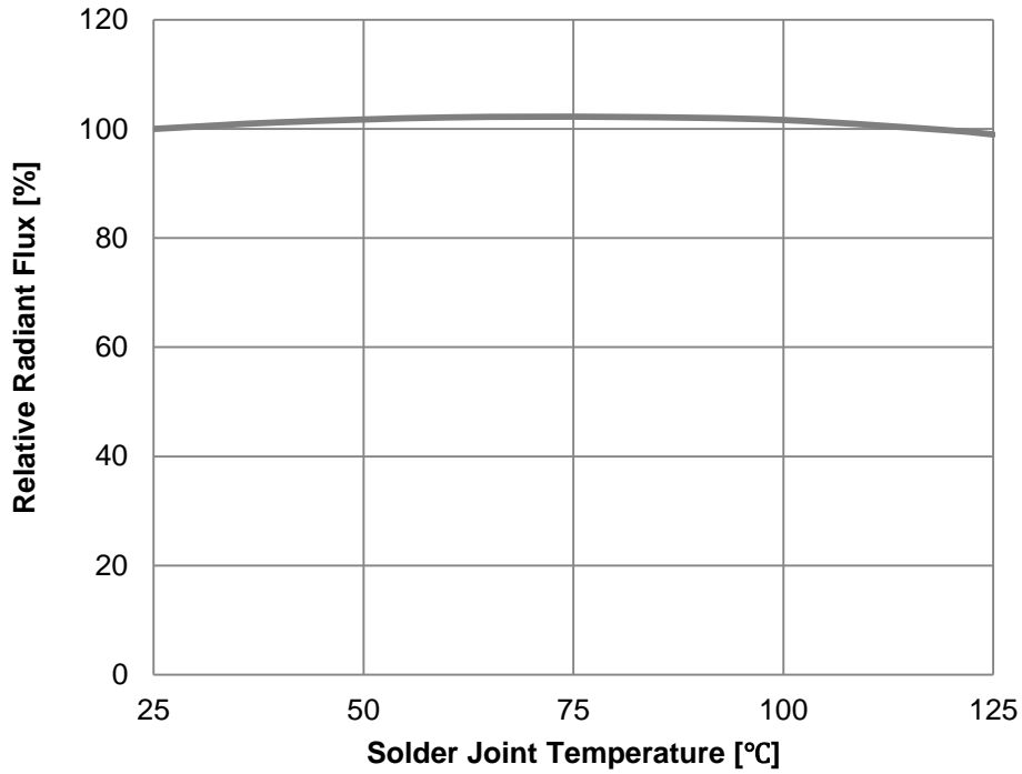
Fig 5. Solder Joint Temperature vs. Relative Radiant Flux, I_F=500\text{mA}
