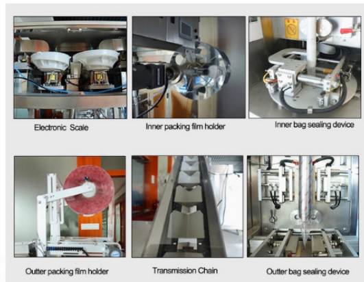
Automatic Triangular Teabag Machine
