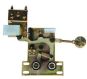
331# PB16D门锁 PB16D door lock
