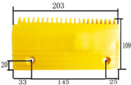
1105# 康力22齿(左) 203×109×孔145 型号: BEVG KONE 22-teeth Comb (Left)
