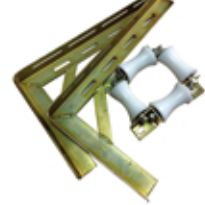
446# 导向装置 Guide Device for Compensation Chain
