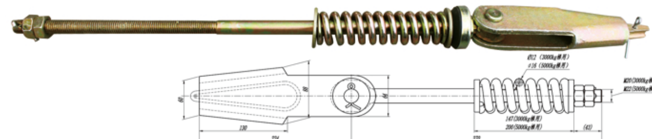
060# 对称锥块式绳头组合 \phi 16 Symmetrical cone block type rope head combination Phi 16
