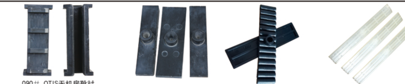
090# OTIS无机房靴衬 100×40×34×12 Otis boots without machine room lining 091# 奥的斯三合一靴衬 Otis three-in-one boot 092# 奥的斯靴衬 长短两种 Otis boots, both short and long 093# 奥的斯靴衬200×25×6 Otis boots
