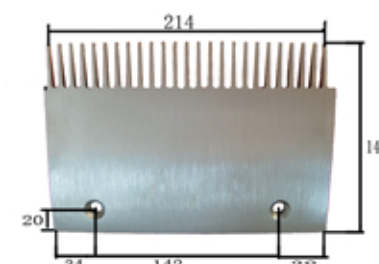
1185# 西子OTIS 25齿人行道铝梳齿板 214×145×孔142 (右) 识别号(Number of Identification) XAA453J 25-teeth aluminium comb plate(right)
