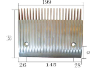
1166# 迅达、富士22齿铝梳齿板 (中) 199×153×孔距145 22-teeth aluminium comb plate 识别号(Number of Identification)DAW-A305004N
