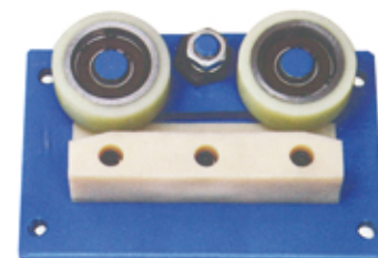
062# 额定速度Rated speed: \leq 0.63\text{m/s} 额定载重量Rated load: \leq 320\text{kg} 导轨宽度Track width: 10, 16mm X方向受力Force in the x direction: \leq 2000\text{N} Y方向受力Force in the Y direction: \leq 2300\text{N}
