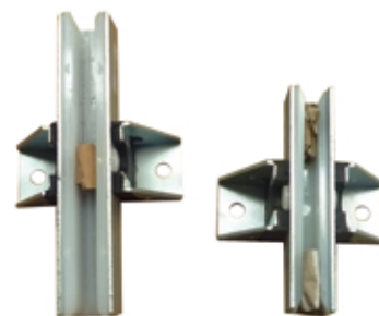
041# OTIS导靴 3种孔90*直径10.5 200*16 (14) 150*10 Otis boot with 3 holes 90 * Diameter 10.5
