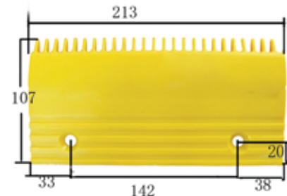
1098# 西子OTIS 25齿塑料梳齿板 (右) 213×107×孔142 识别号(Number of Identification) LDTJ-B-1 25-teeth plastic comb plate (right)
