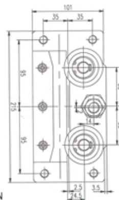
060# 额定速度Rated speed: \leq 0.63\text{m/s} 额定载重量Rated load: \leq 320\text{kg} 导轨宽度Track width: 10, 16mm X方向受力Force in the x direction: \leq 1600\text{N} Y方向受力Force in the Y direction: \leq 1500\text{N}
