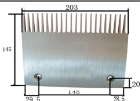
1188# 西子OTIS 22齿铝梳齿板 (右) 203×145×孔145 22-teeth aluminium comb plate (right)
