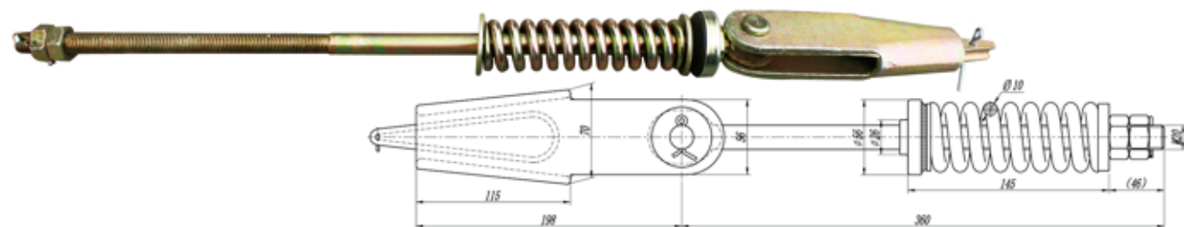
061# 对称锥块式绳头组合 \phi 13 Symmetrical Cone Block Rope Head Combination Phi 13
