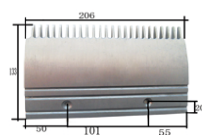
1180# OTIS 24齿铝梳齿板 (左) 206×133×孔距101 识别号(Number of Identification) 56-XAA453BJ 24-teeth aluminium comb plate(left)
