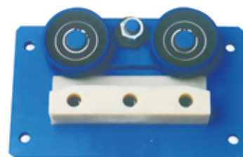
061# 额定速度Rated speed: \leq 0.4\text{m/s} 额定载重量Rated load: \leq 320\text{kg} 导轨宽度Track width: 10, 16mm
