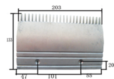
1181# OTIS 24齿铝梳齿板 (中) 203×133×孔距101 识别号 Number of Identification 56-XAA453BJ 24-teeth aluminium comb plate(centre)
