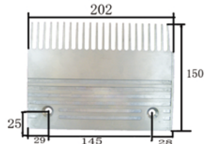
1173# 江南22齿铝梳齿板(右) 202×150×孔145 22-teeth aluminium comb plate(right)
