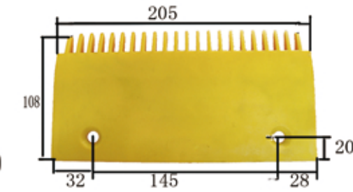
1115# 迅达22齿塑料梳齿板 (边) 205×108×孔145 22-teeth plastic comb plate( left )
