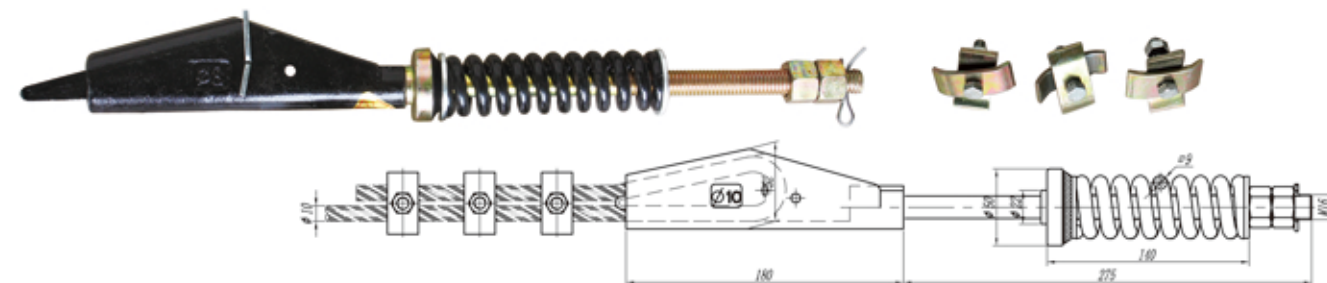
066# (SLBJ-4) 非对称楔块绳头组合 \phi 10 Asymmetric Wedge Rope Head Combination Phi 10
