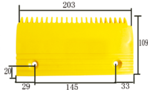
1107# 康力梳齿板(右) 型号: BEVG KONE 22-teeth COMB (Right)
