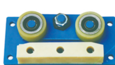
060# 额定速度Rated speed: \leq 0.63\text{m/s} 额定载重量Rated load: \leq 320\text{kg} 导轨宽度Track width: 10, 16mm X方向受力Force in the x direction: \leq 1600\text{N} Y方向受力Force in the Y direction: \leq 1500\text{N}
