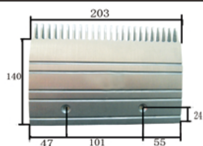
1178# OTIS 24齿铝梳齿板 203×140×孔距101 24-teeth aluminium comb plate 识别号(Number of Identification)XAA453CD
