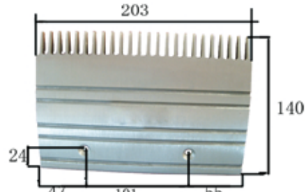
1175# OTIS、LG 24齿铝梳齿板 203×140×孔101 (中) 识别号(Number of Identification) GAA453BM 24-teeth aluminium comb plate(centre)
