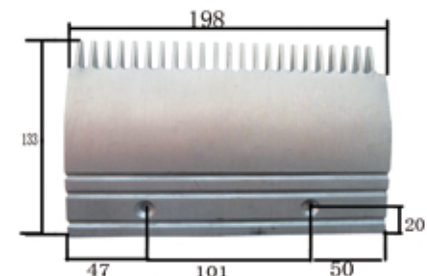
1182# OTIS 23齿铝梳齿板 (右) 198×133×孔距101 识别号(Number of Identification) 56-XAA453BJ 23-teeth aluminium comb plate(right)
