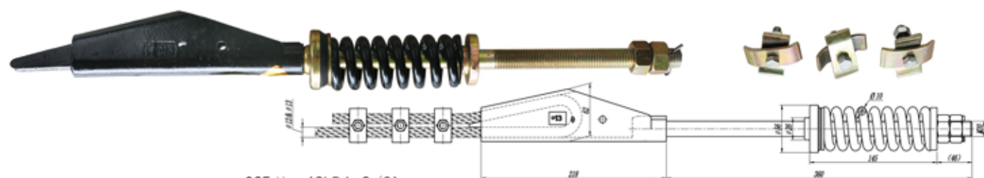
065# (SLBJ-2/3) 非对称楔块绳头组合 \phi 12/13 Asymmetric Wedge Rope Head Combination Phi 12/13
