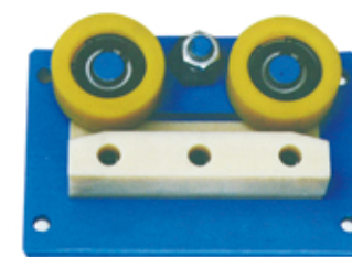
063# 额定速度Rated speed: \leq 0.63\text{m/s} 额定载重量Rated load: \leq 450\text{kg} 导轨宽度Track width: 10, 16mm X方向受力Force in the x direction: \leq 2000\text{N} Y方向受力Force in the Y direction: \leq 2300\text{N}
