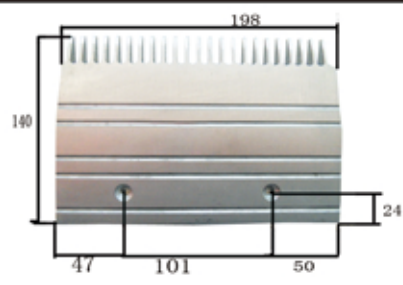
1179# OTIS 23齿铝梳齿板 198×140×孔距101 23-teeth aluminium comb plate 识别号(Number of Identification) GAA453BM
