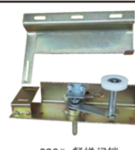
630# 餐梯门锁 Dining ladder door lock
