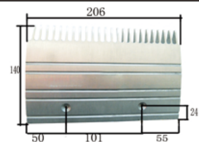
1177# OTIS 24齿铝梳齿板 206×140×孔距101 识别号(Number of Identification) GAA453BM
