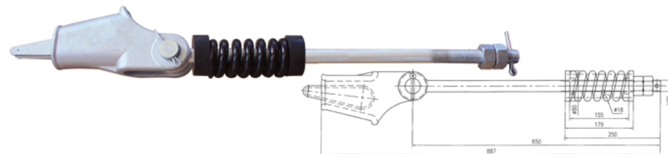
068# (SLBJ-8) 对称楔块式绳头组合 \phi 19 Symmetrical Wedge Rope Head Combination Phi 19
