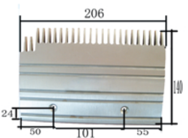
1174# OTIS、LG 24齿铝梳齿板 206×140×孔距101 (左) 识别号(Number of Identification) GAA453BM 24-teeth aluminium comb plate(left)
