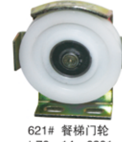
621# 餐梯门轮 \phi 76 \times 14 \times 6201 Dining ladder door wheel
