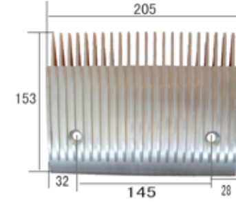
1165# 迅达、富士22齿铝梳齿板 (边) 205×153×孔距145 22-teeth aluminium comb plate 识别号(Number of Identification)DAW-A305004N
