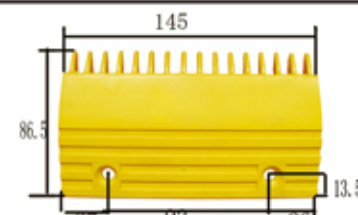
1094# 现代16齿ABS梳齿板(中) 145×86.5×孔距92 识别号(Number of Identification) HE655B013 16-teeth ABS comb plate (centre)
