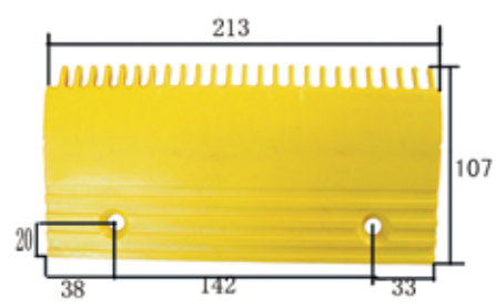
1096# 西子OTIS 25齿塑料梳齿板 (左) 213×107×孔142 识别号(Number of Identification) LDTJ-B-2 25-teeth aluminium comb plate(left)
