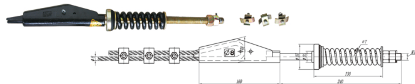
067# (SLBJ-5) 非对称楔块绳头组合 \phi 8 Asymmetric wedge rope head combined Phi 8
