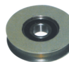
246# 客梯门挂轮 φ 66 × 15 × 6202 Passenger elevator door hanging wheel
