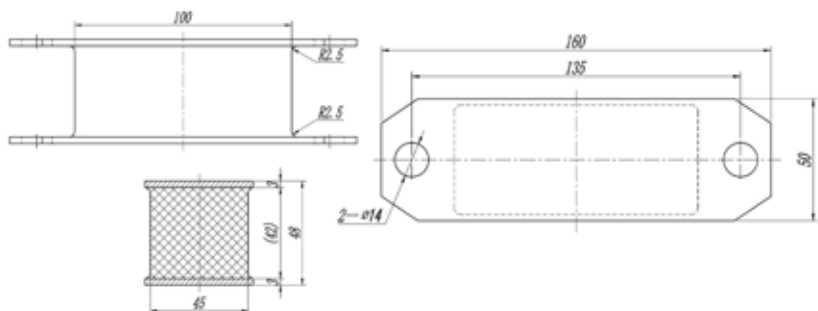
421# (SLBJ-166/C) 轿厢称重件 Car weighing piece
