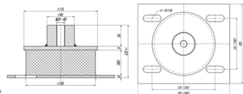
424# (SLBJ-168/B) 曳引机减震垫 Traction machine damping pad
