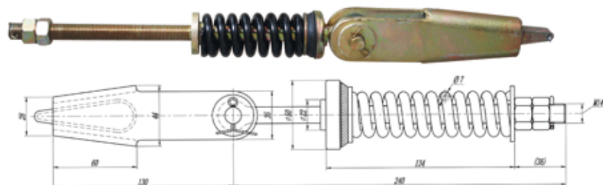
063# 对称锥块式绳头组合 \phi 8 Symmetrical cone block type rope head combined Phi 8
