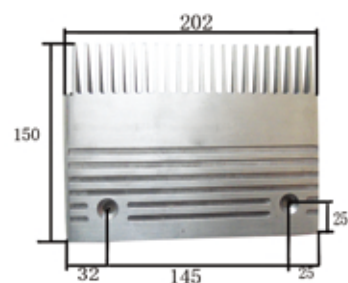
1171# 江南22齿铝梳齿板(左) 202×150×孔145 22-teeth aluminium comb plate(left)
