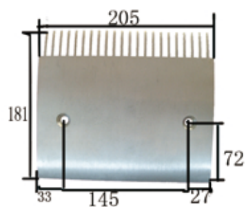
1168# 迅达22齿铝梳齿板 205×181×孔距145 (边) 22-teeth aluminium comb plate(side)
