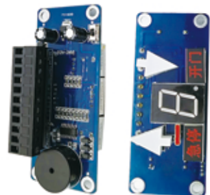
650# 手接线显示板 Hand-wired display panel
