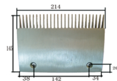
1183# 西子OTIS 25齿人行道铝梳齿板 214×145×孔142 (左) 识别号(Number of Identification) XAA453J 25-teeth aluminium comb plate(left)
