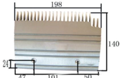
1176# OTIS、LG 23齿铝梳齿板 198×140×孔102 (右) 识别号(Number of Identification) GAA453BM 23-teeth aluminium comb plate(right)
