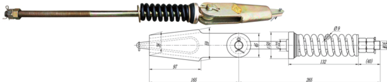
062# 对称锥块式绳头组合 \phi 10 Symmetrical cone block type rope head combined Phi 10
