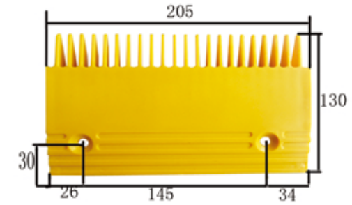
1112# 东芝22齿ABS梳齿板 (右) 205×120×孔145 22-teeth ABS comb plate (right)
