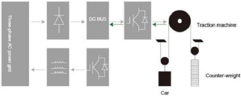
Working diagram of energy feedback system
