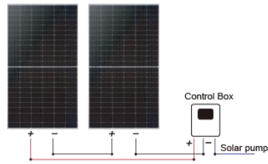
2 Solar panel: 2 Pcs x (50 ~ 100W)
