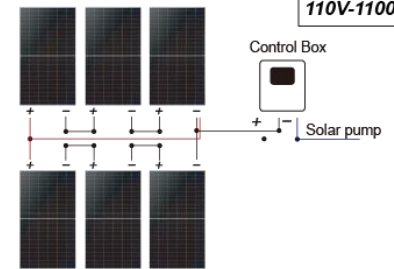
3 Solar panel: 6 Pcs x (200 ~ 350W)
