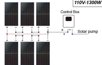
3 Solar panel: 6 Pcs x (300 ~ 450W)
