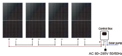
1 Solar panel: 4 Pcs x (350 ~ 650W)
