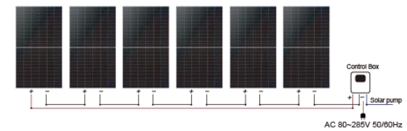
2 Solar panel: 6 Pcs x (300 ~ 400W)
