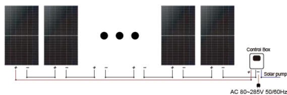
1 Solar panel: 7 Pcs x (400 ~ 650W)
