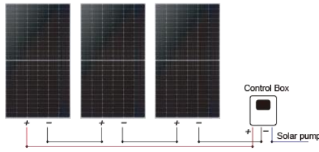
2 Solar panel: 3 Pcs x (350 ~ 550W)
