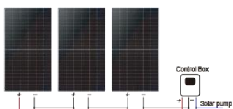
1 Solar panel: 3 Pcs x (550 ~ 650W)
