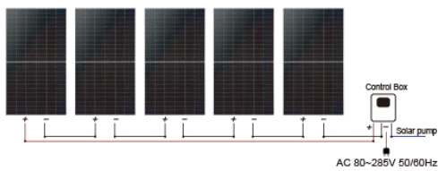
1 Solar panel: 5 Pcs x (400 ~ 650W)
