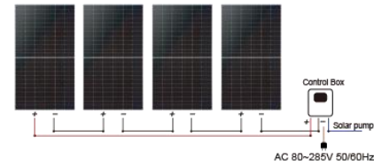
2 Solar panel: 4 Pcs x (250 ~ 350W)
