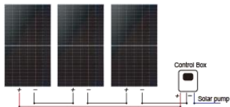
1 Solar panel: 2 Pcs x (400 ~ 500W)
