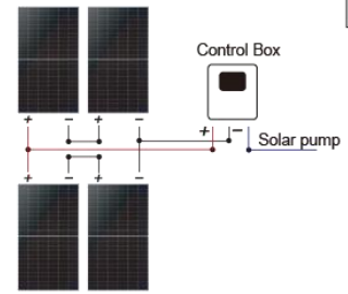
3 Solar panel: 4 Pcs x (250 ~ 350W)
