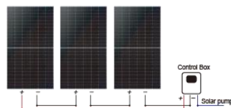
1 Solar panel: 3 Pcs x (500 ~ 650W)
