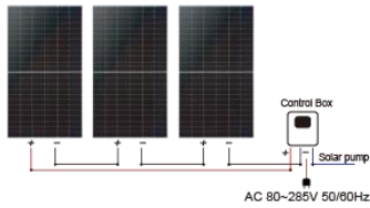
1 Solar panel: 3 Pcs x (350 ~ 650W)
