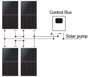
1 Solar panel: 4 Pcs x (350 ~ 550W)
