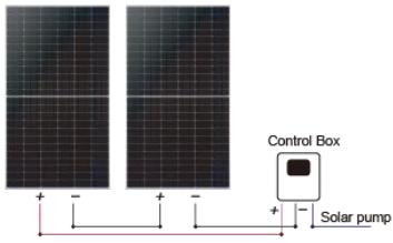
1 Solar panel: 2 Pcs x (550 ~ 650W)
