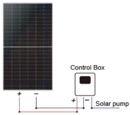
1 Solar panel: 1 Pcs x (100 ~ 200W)
