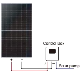
1 Solar panel: 1 Pcs x (250 ~ 550W)
