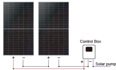
2 Solar panel: 2 Pcs x (80 ~ 150W)
