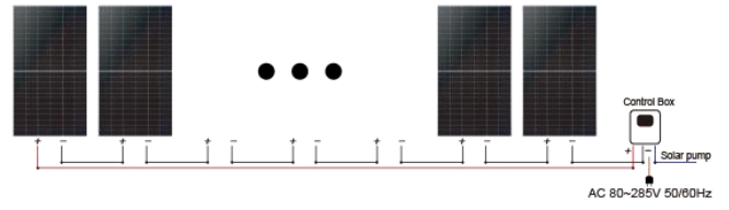
❷ Solar panel: 9 Pcs x (350 ~ 400W)
