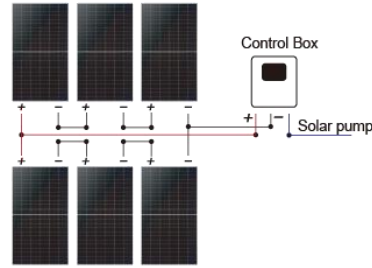
2 Solar panel: 6 Pcs x (250 ~ 350W)
