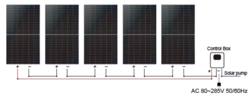
2 Solar panel: 5 Pcs x (250 ~ 350W)
