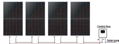
2 Solar panel: 3 Pcs x (300 ~ 400W)
