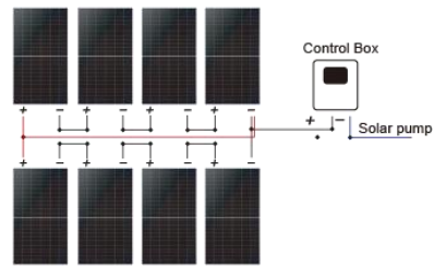
2 Solar panel: 8 Pcs x (250 ~ 500W)
