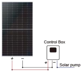
1 Solar panel: 1 Pcs x (150 ~ 250W)
