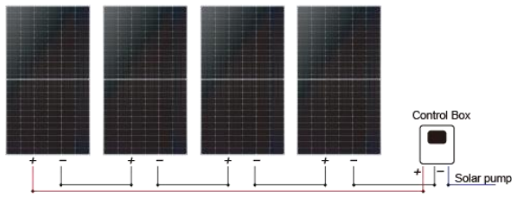
1 Solar panel: 4 Pcs x (500 ~ 650W)
