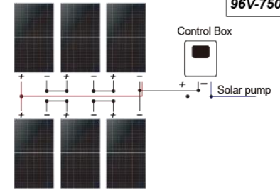
3 Solar panel: 6 Pcs x (200 ~ 300W)
