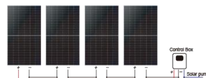
2 Solar panel: 4 Pcs x (450 ~ 550W)
