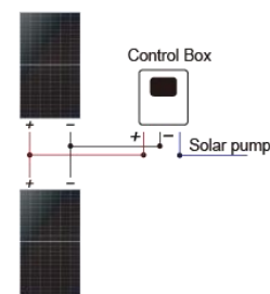
2 Solar panel: 2 Pcs x (200 ~ 380W)
