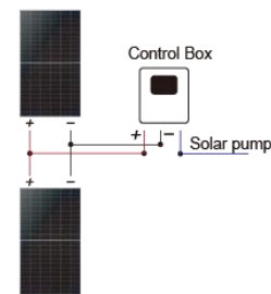
2 Solar panel: 2 Pcs x (120 ~ 250W)
