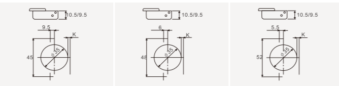
铰杯种类 (Hinge cup types)
