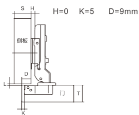
(Half cover 半盖)
