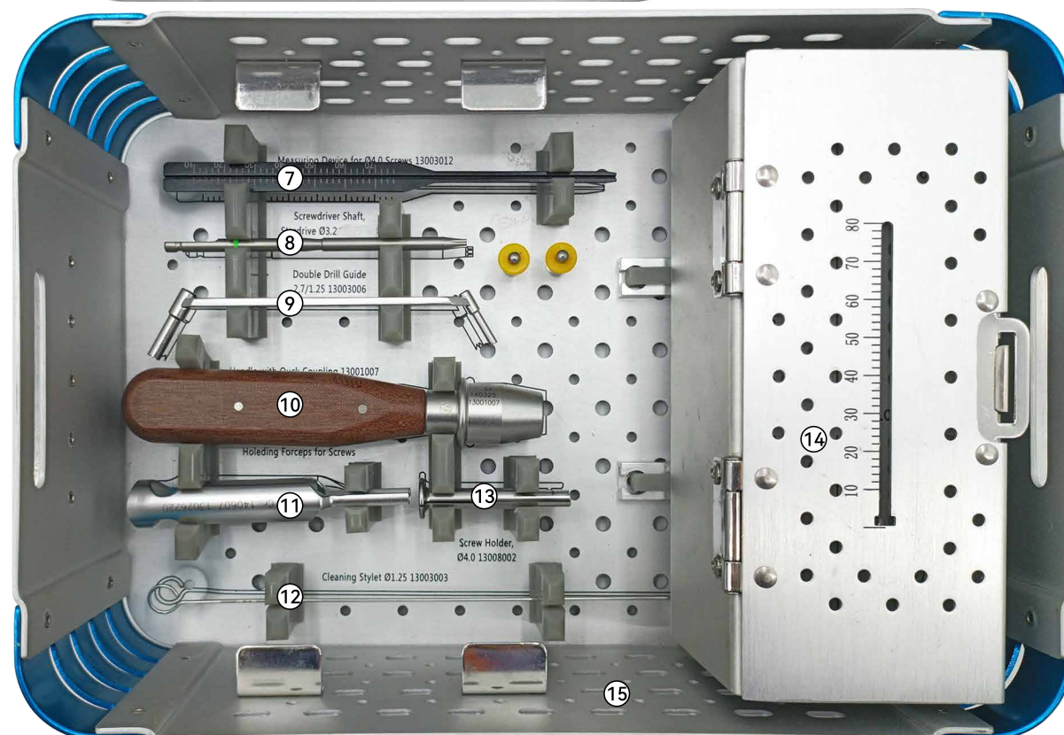
13008991 Screw Case
