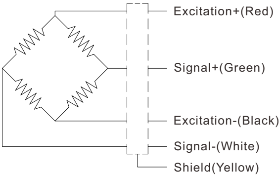
Wiring Code@Compression
