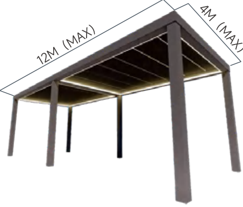
Six - Posts
