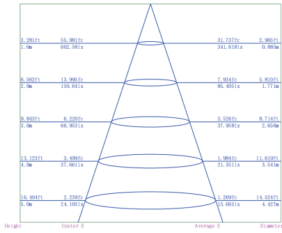
Illumination Picture ( 20°x50°)
