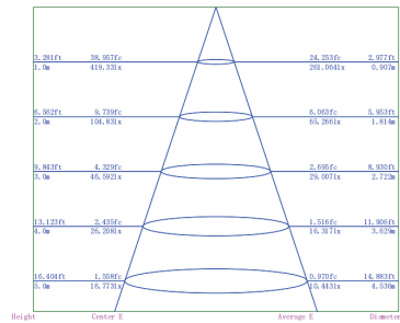
Lux distance Curve (3000K, 20°x45°)
