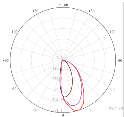
Lux distance Curve (3000K, 20°x50°)
