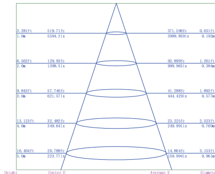
Illumination Picture ( 10° )
