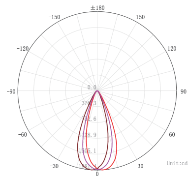
Lux distance Curve (3000K, 36° )
