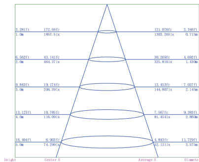
Illumination Picture ( 36° )
