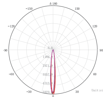
Lux distance Curve (3000K, 10° )
