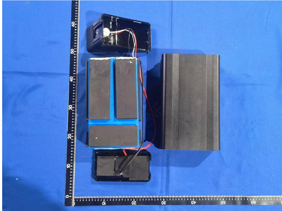
Picture 3 Internal view-1 of battery
