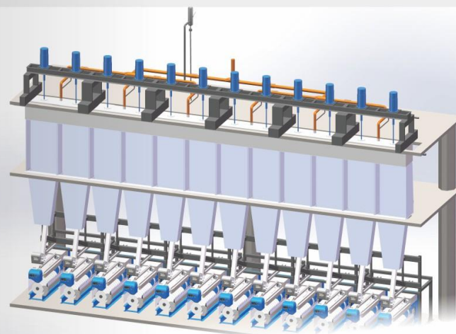
ZKBP612A-180型高速卷绕头 Zkbp612a-180 High-speed Winder
