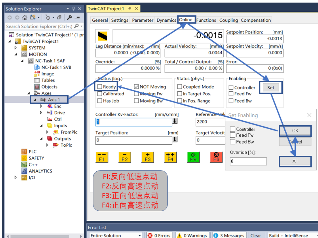
图7-14 NC 轴点动
