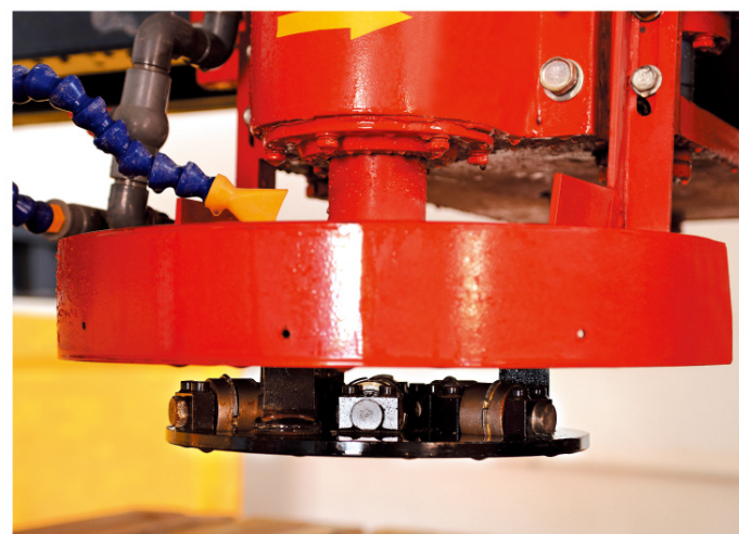
Bridge Cutter
