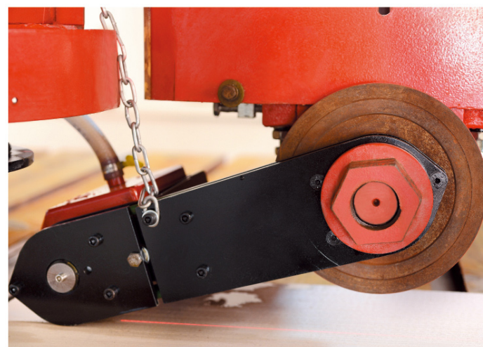
Roller Transmission
