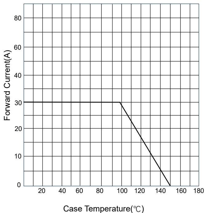
FIG 1: I_F - T_C
