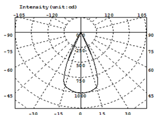
Intensity data:(deg , cd) CO-180
