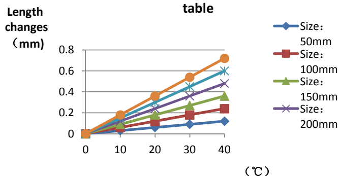
PMMA product size changes with temperature table
