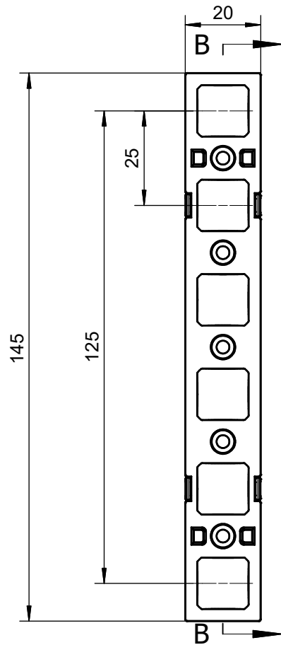
LED基板上表面 Top surface of LED substrate
