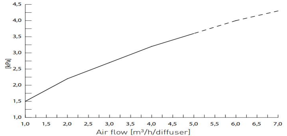
Wet pressure loss
