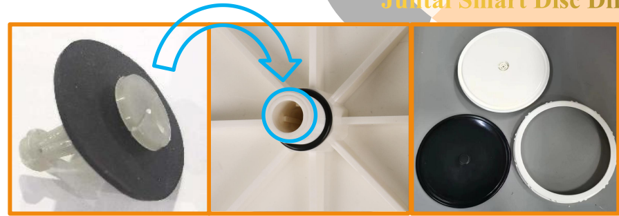
Multiple Check Valves
