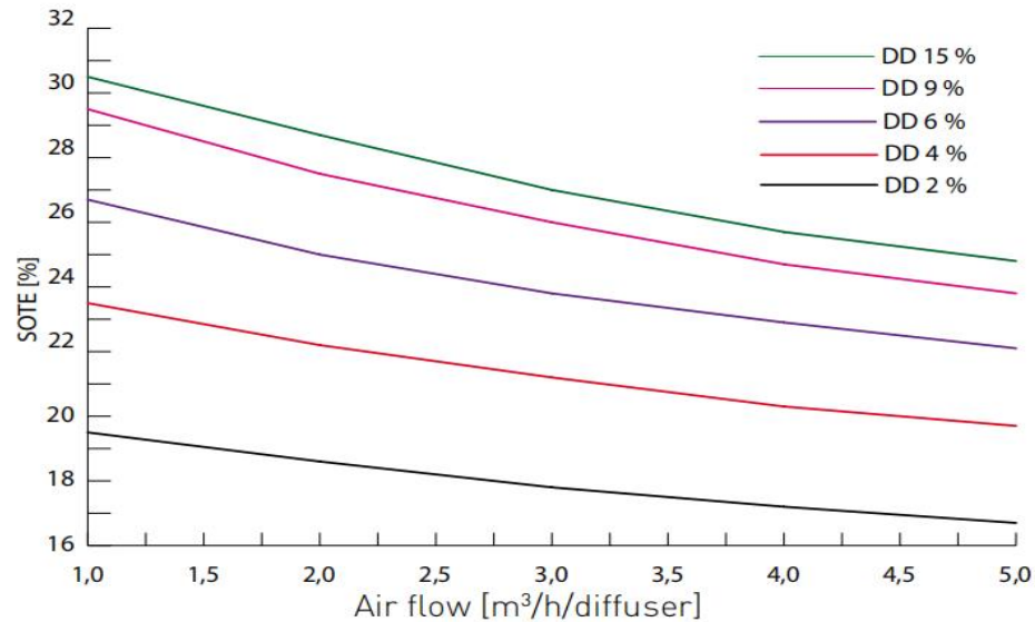
Standard oxygen transfer efficiency, SOTE
