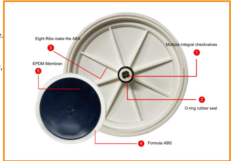
Multiple Check Valves
