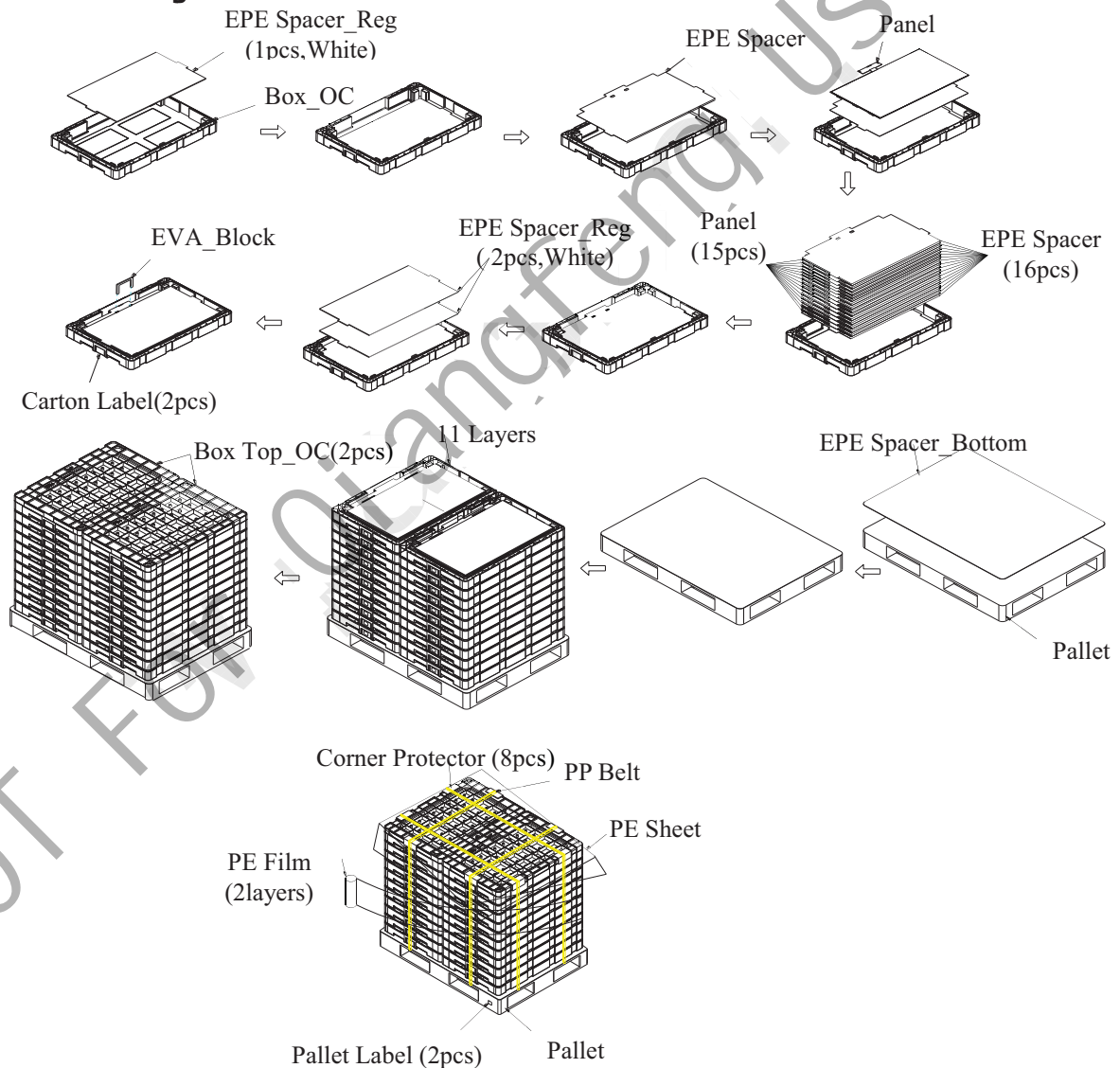
Fig. 7.1 Packing method
