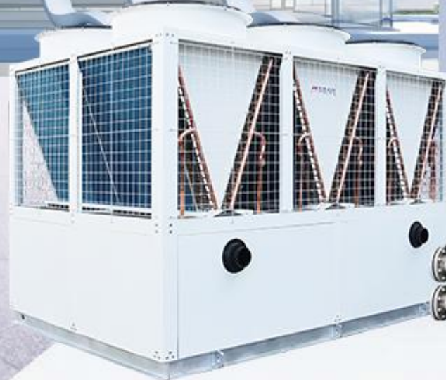
Low ambient temperature air-cooled large scroll unit
