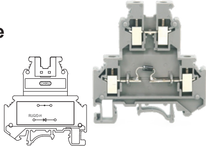
RUG/D-H
