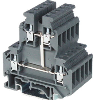
RTB 4-L/LB-PV
