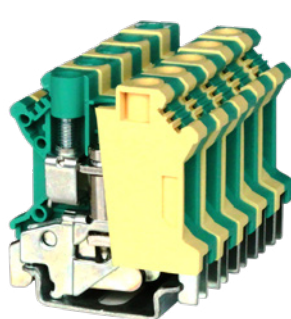
RTB 6-PE
