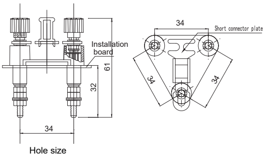
RP 1-3 Installation diagram
