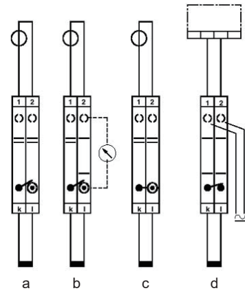
simple current transformer test circuit
