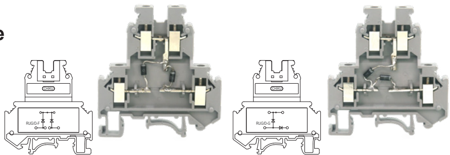
RUG/D-F
