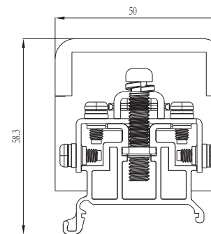
RMJ 2.5
