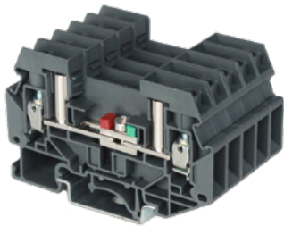
RTB 6-RTK/S
