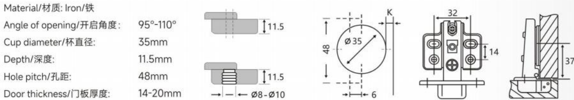
AF826 3D06 Aluminum Frame 3D Gun Black Hinge with 6 hole
