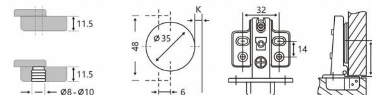
GC3D04 SS or Iron 3D Hydraulic hinge
