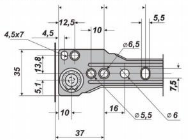
外轨头部孔位: Drilling pattern for cabinet member
