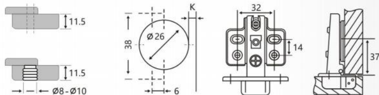
26G Small Iron Hydraulic/Normal Glass Door Hinge
