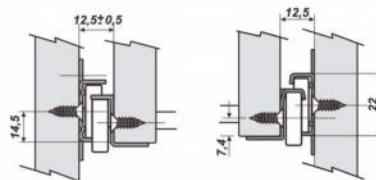
装配尺寸: Installation measurement
