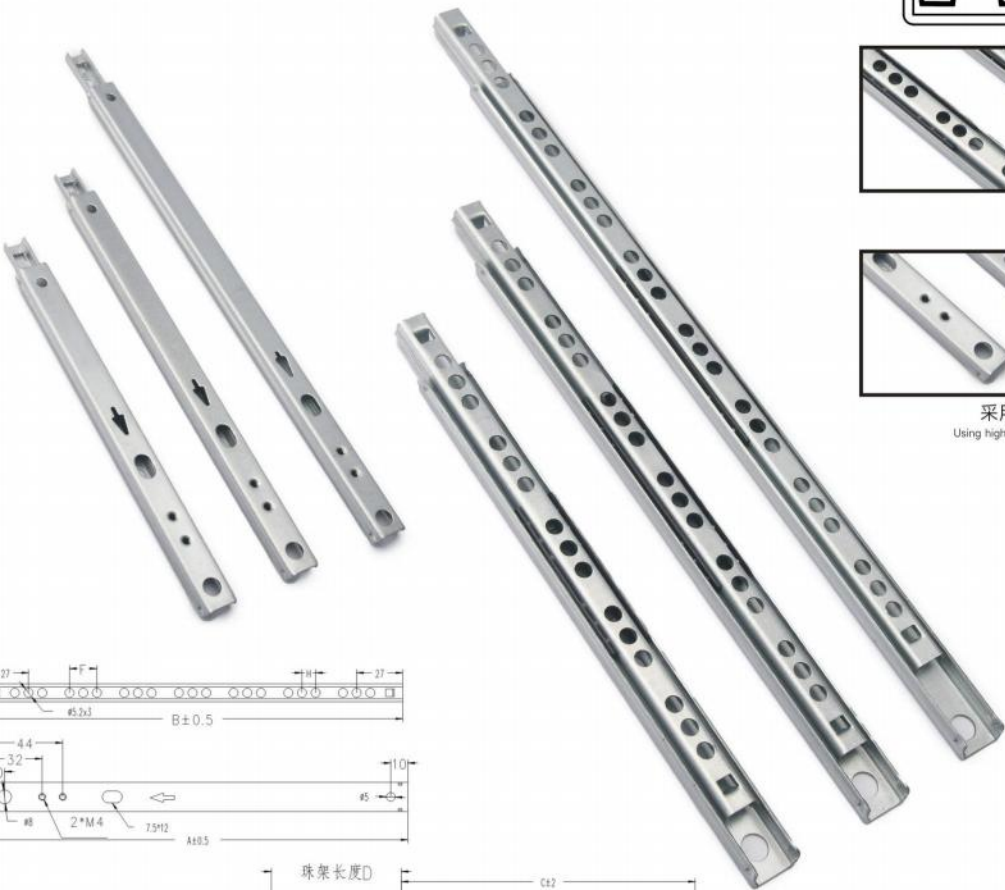
消声钢珠 Muffled ball
