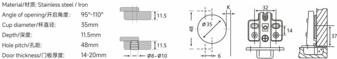
SA2 Iron Short Arm Hinge With 2D screw
