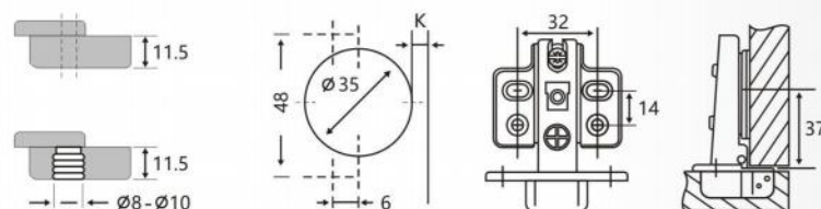
GCN863 Half SS Hydraulic Hinge
