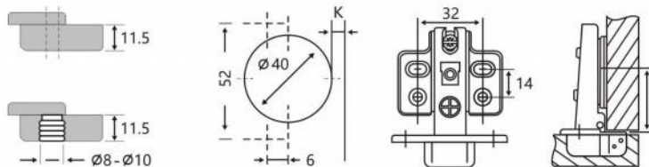
GC401 Slide-on Iron Hydraulic Hinge
