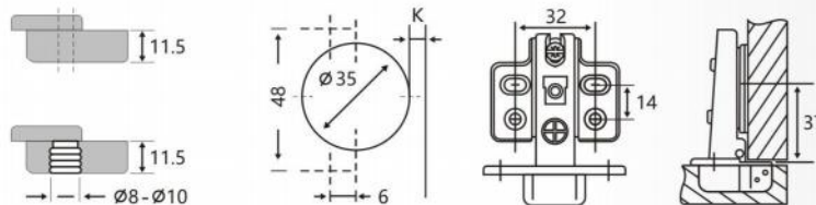
AFSS SS Hydraulic Hinge With Hook
