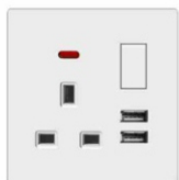
A5-021 13A switched socket+2USB w/without neon(single pole) A5-022 13A switched socket+2USB w/without neon(double pole)
