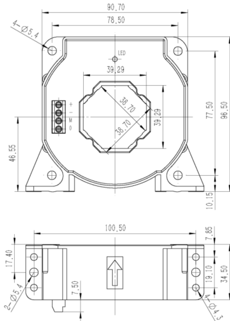
Figure 1: Outline Drawing
