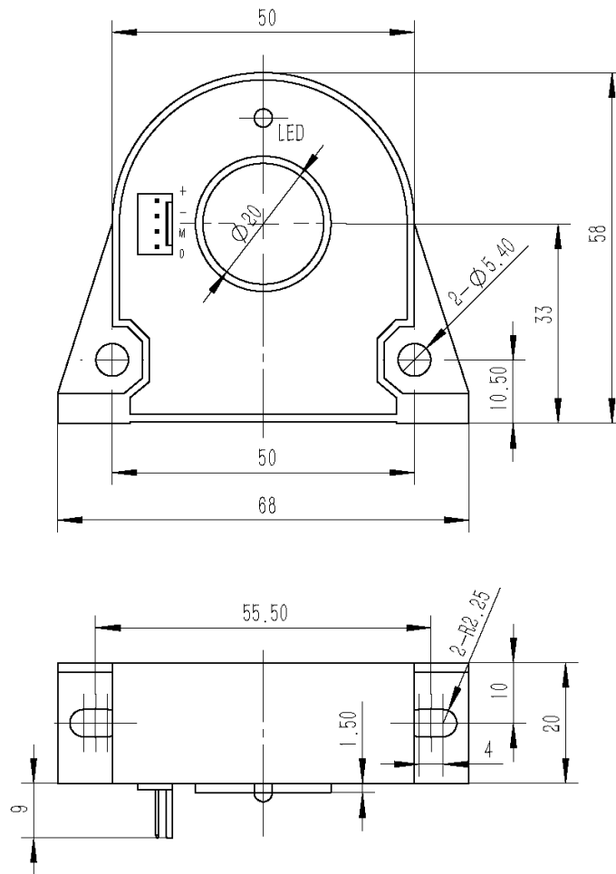
Figure 1: Outline Drawing
