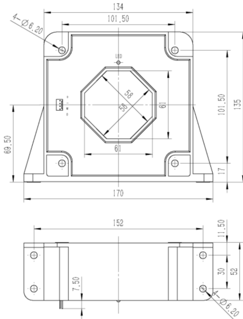
Figure 1: Outline Drawing
