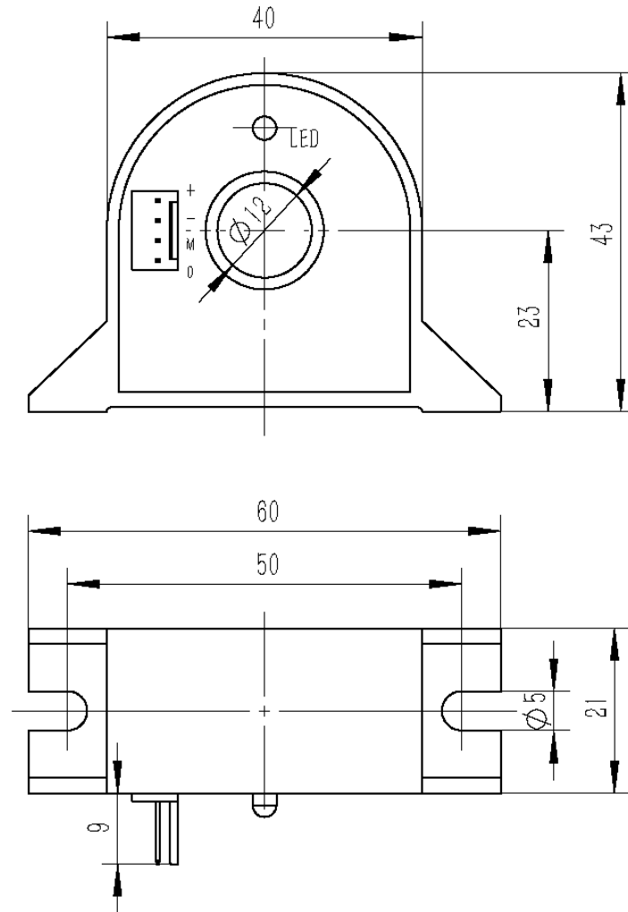
Figure 1: Outline Drawing
