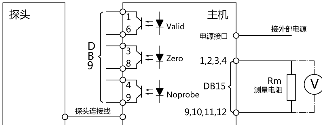
Electrical connection
