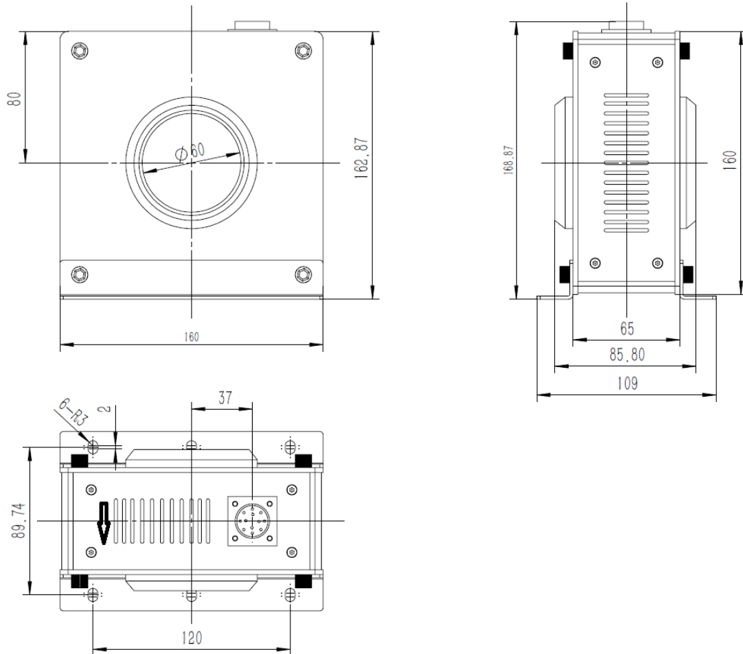
Figure 2: Probe Dimensions
