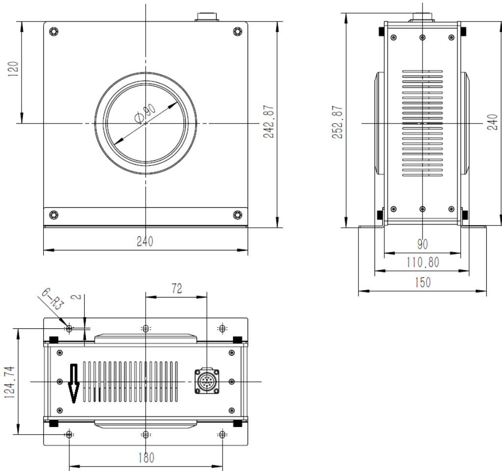
Figure 2: Probe Dimensions
