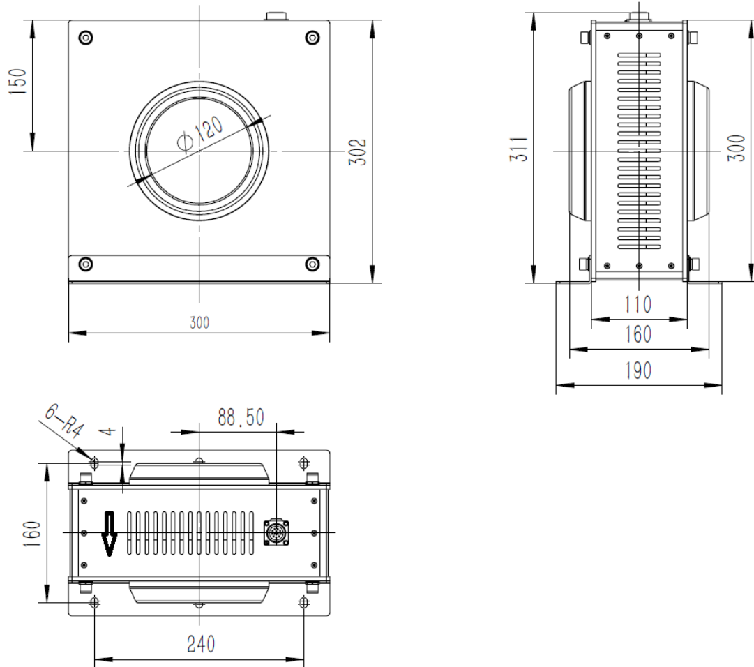
Figure 2: Probe Dimensions
