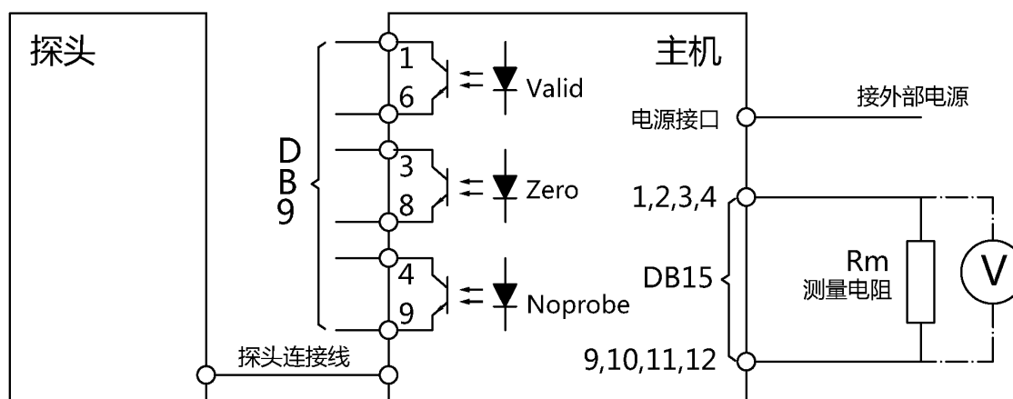
Electrical connection
