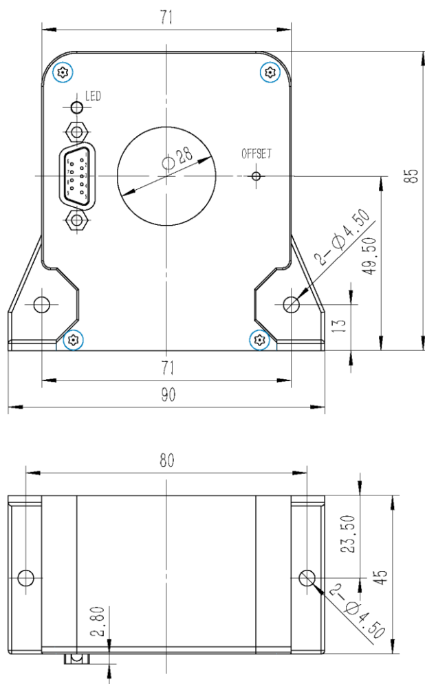
Figure 1: Dimensions
