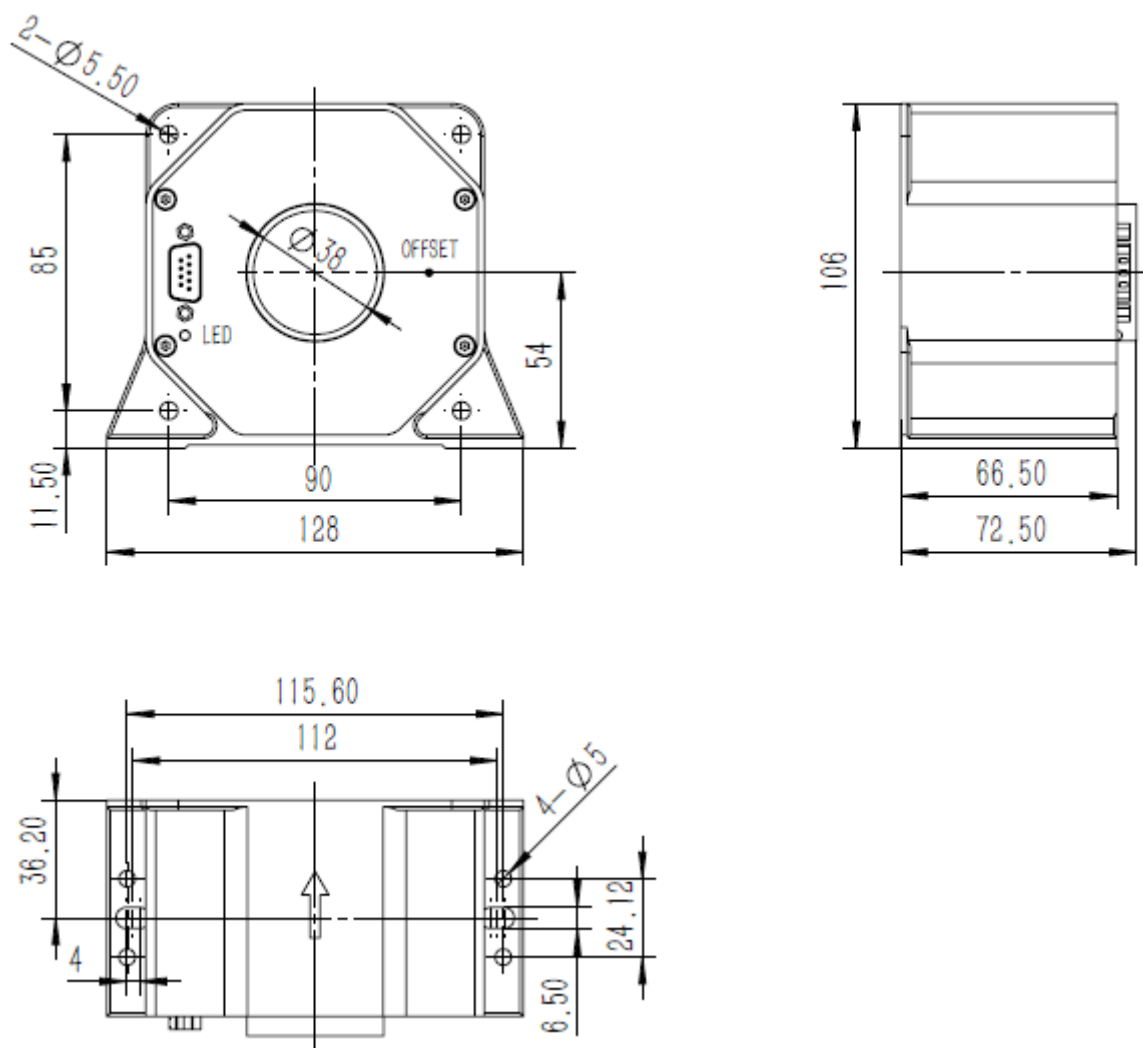
Figure 1: Dimensions
