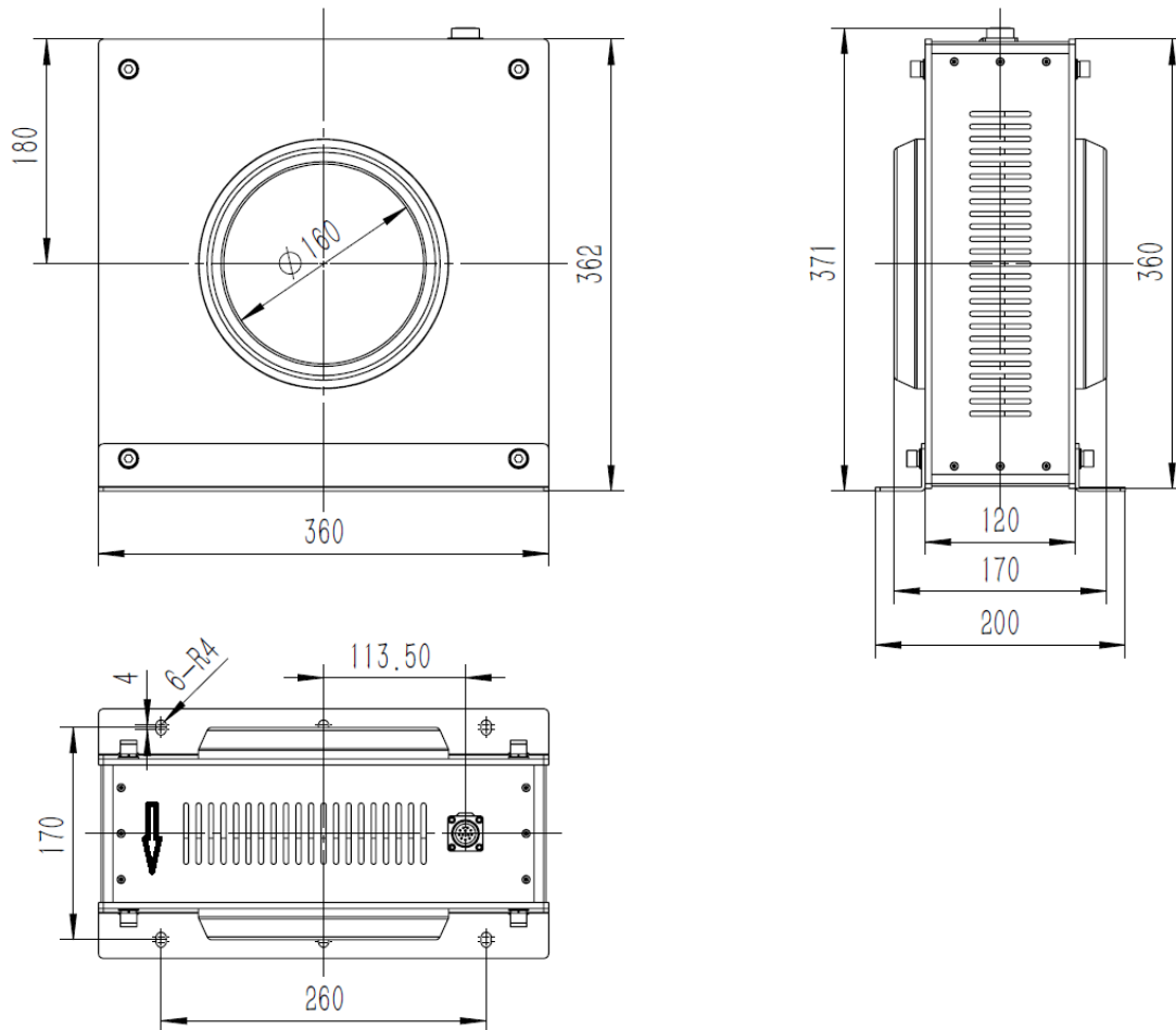
Figure 2: Probe Dimensions
