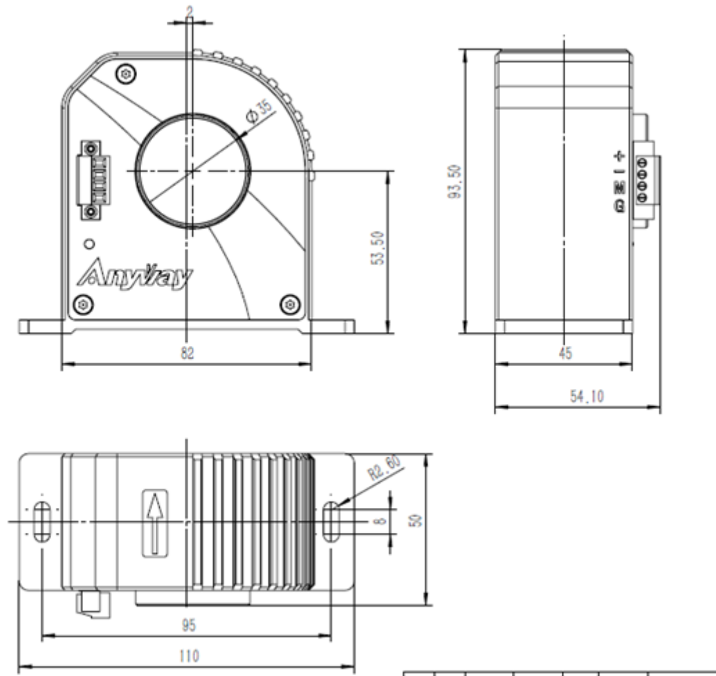
Figure 1: Outline Drawing
