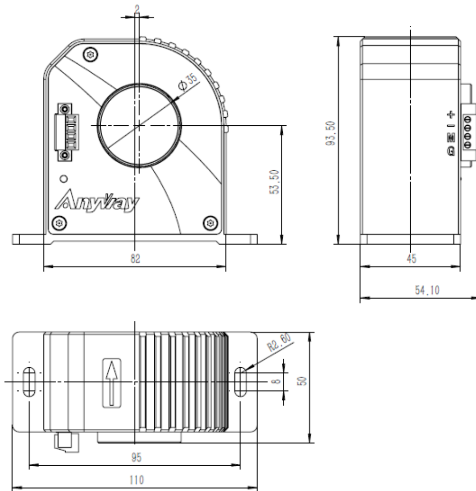
Figure 1: Outline Drawing
