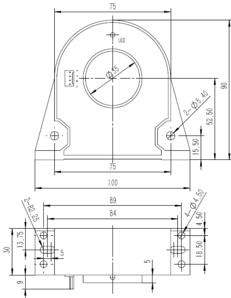
Figure 1: Outline Drawing
