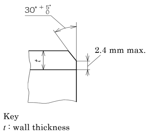
Figure 1 Shape of bevel end
