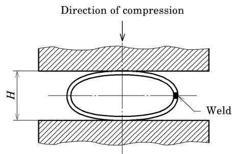
Figure 2 Flattening test
