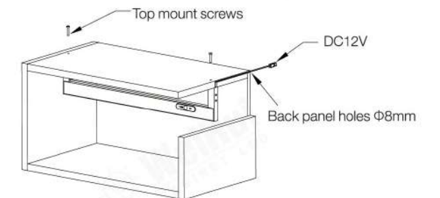
Top Installation
