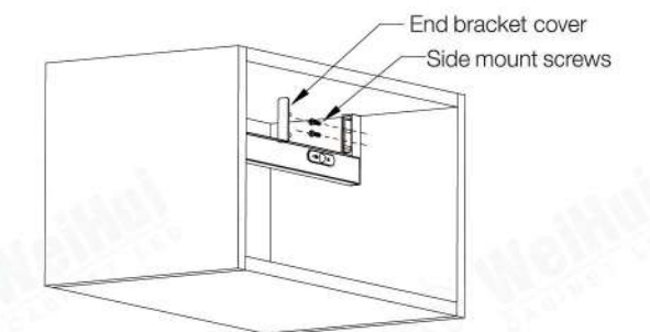
Side Installation
