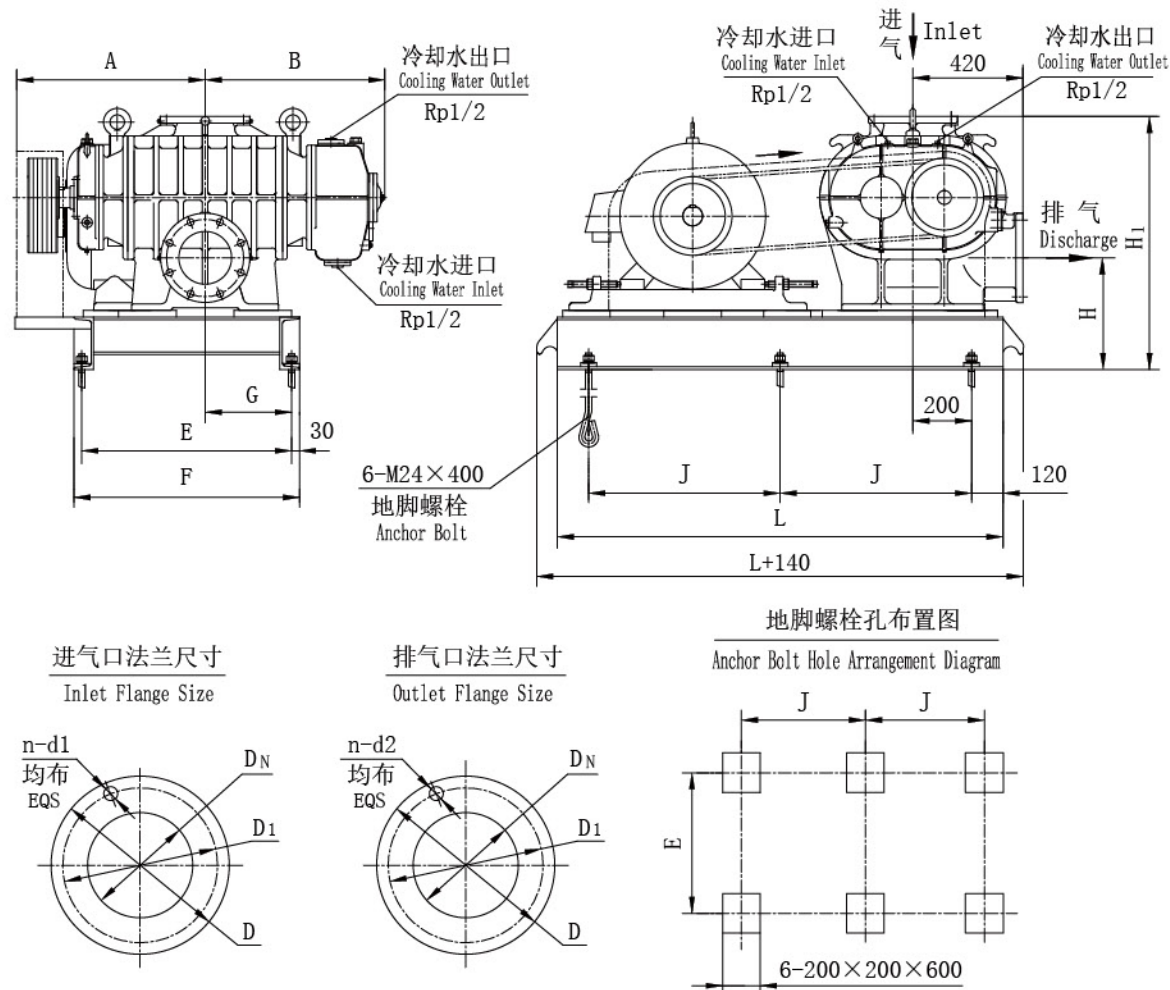
3HE型罗茨鼓风机皮带传动外形图 BELT DRIVE OUTLINE DRAWING FOR MODEL 3HE ROTARY BLOWER
