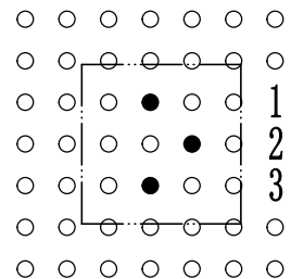
Terminal Spacing on a 2.54 PCB
