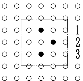
Terminal Spacing on a 2.54 PCB
