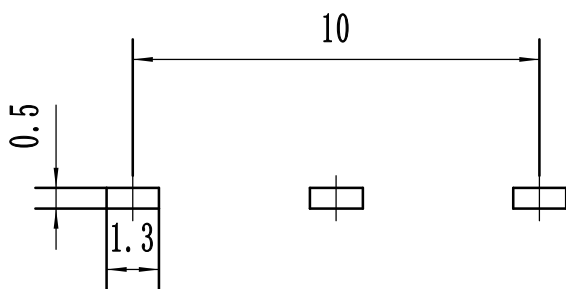
Terminal Spacing on a PCB
